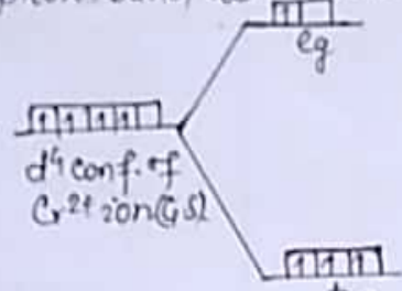
In octahedral ligand field (Strong).
