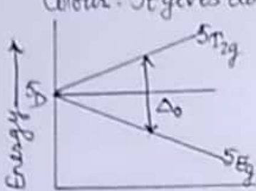
Energy level splitting of d^1 system
