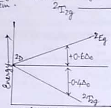
Octahedral ligand field (Orgel diagram of d^1 system/ Ti^{3+} ion)
