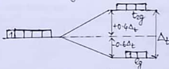
(Tetrahedral ligand field)
